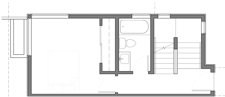
TH 4 - Level 1
