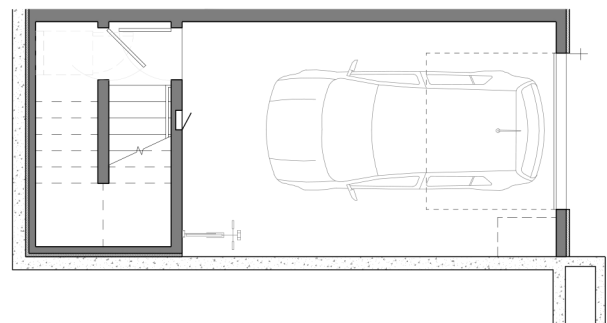
TH 3 - Level 0
