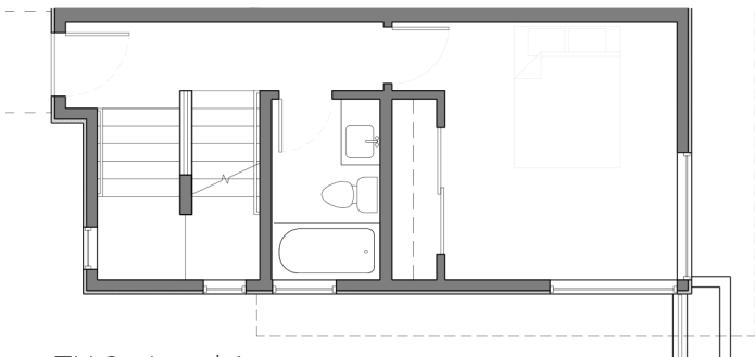
TH 3 - Level 1
