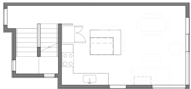
TH 3 - Level 2
